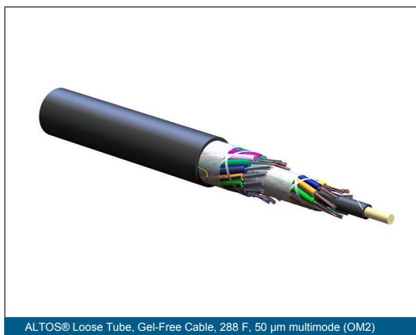
ALTOS® Loose Tube, Gel-Free Cable, 288 F, 50 µm multimode (OM2)
