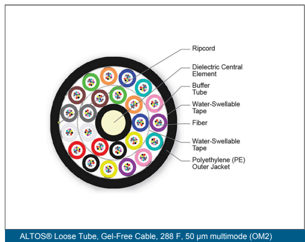
ALTOS® Loose Tube, Gel-Free Cable, 288 F, 50 µm multimode (OM2)
